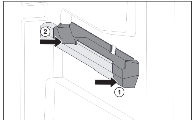
Fig. 51 Attachment on the right moulded rib
